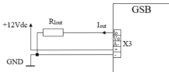
Figure 2 connection circuit
