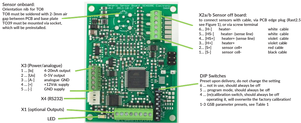
Figure 4 GSB main interfaces and DIP-switches
