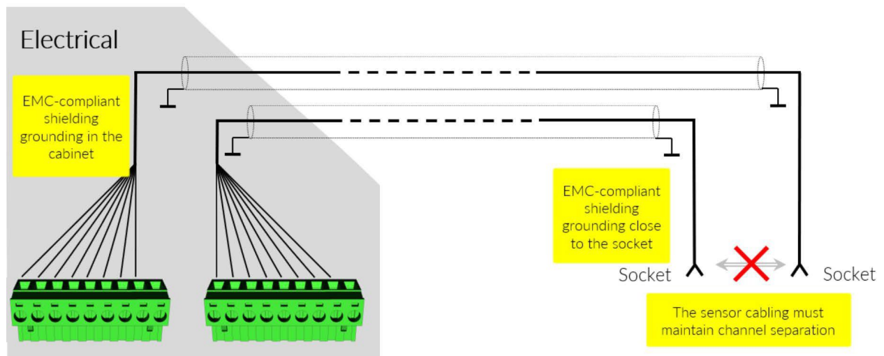
Figure 6. Shielding Grounding
