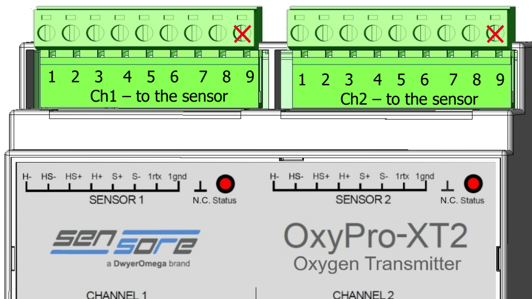
Figure 5. Sensor Side Connections
