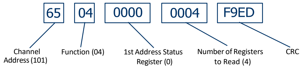
Figure 9. Hexadecimal data packet sent via Modbus function 04 (ppm)
