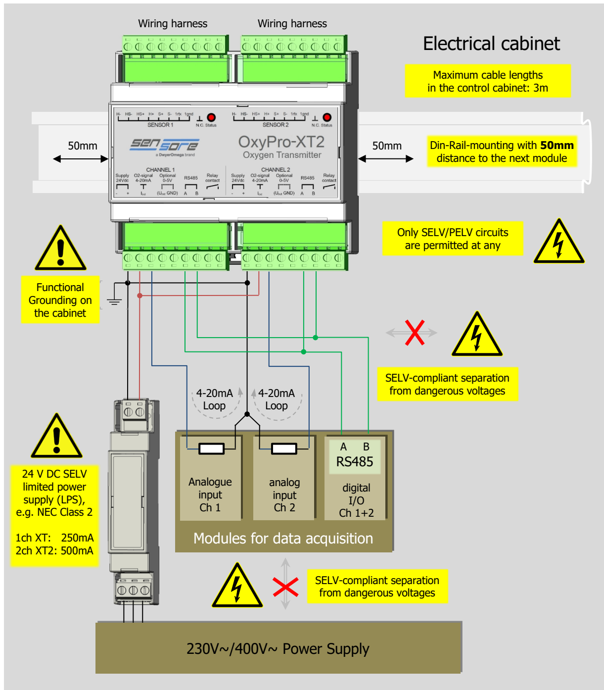
Figure 3. Control Cabinet Connections
