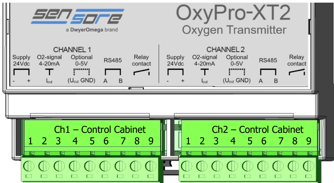
Figure 4. Cabinet side connections
