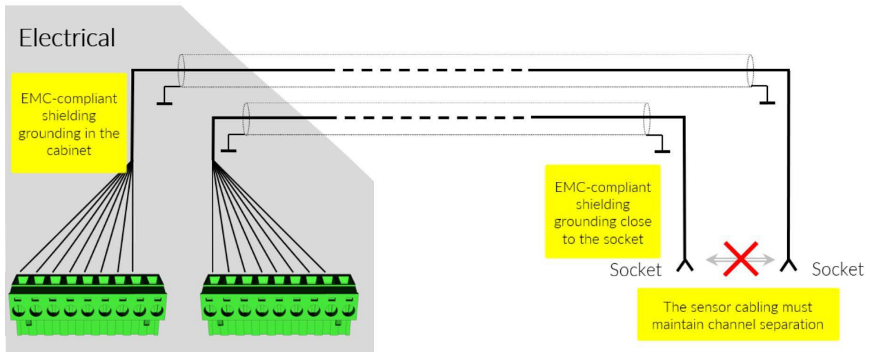
Figure 6. Shielding Grounding
