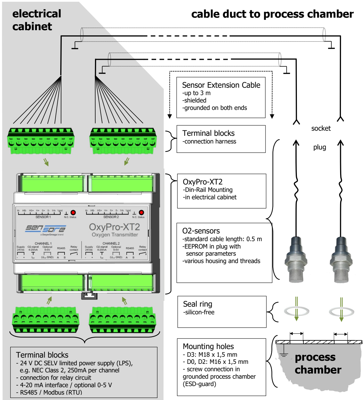
Figure 1. Larger System schematic
