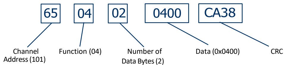
Figure 8. Received hexadecimal data packet via Modbus function 0x04
