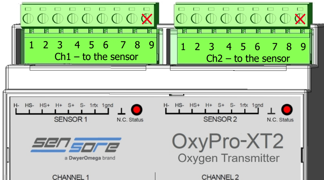
Figure 5. Sensor Side Connections
