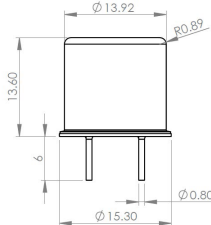
Pin-Side view
